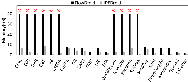
Fig. 9. Comparing IDEDROID and FLOWDROID (in its default setting) in terms of memory consumed. ⊗ indicates apps where FLOWDROID either timed out or exhausted memory resources.
